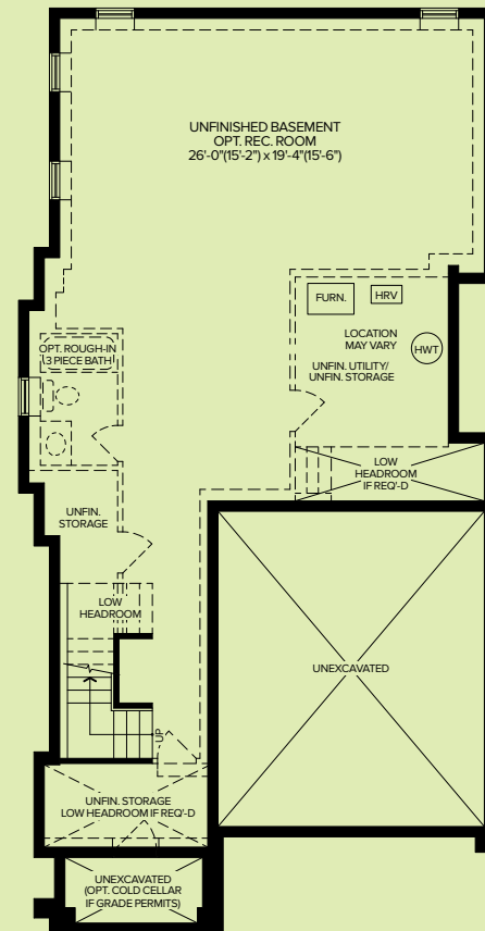
BASEMENT | ELEVATION C
